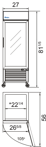
MCF8722GR
