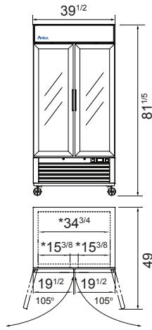
MCF8733GR
