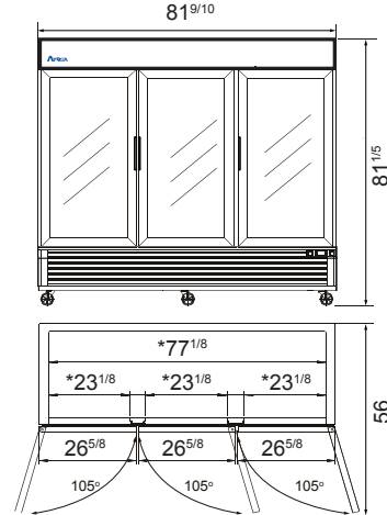
MCF8724GR
