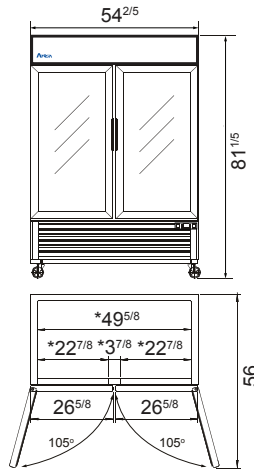
MCF8723GR
